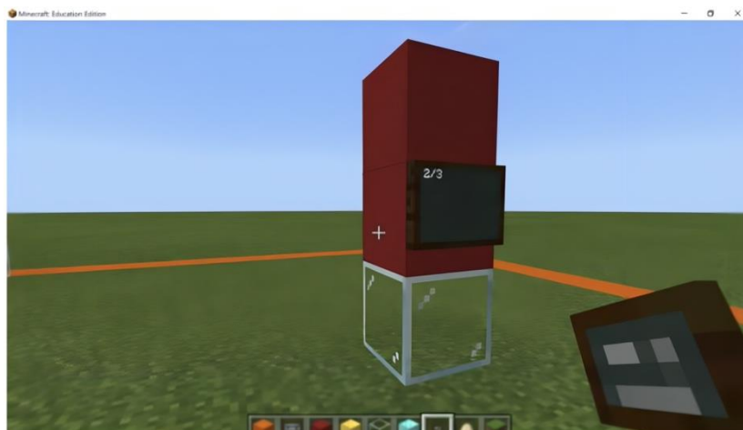
Figure 1 Fraction model with the value of 2/3
